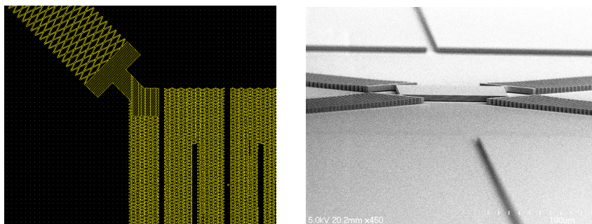
Figure 1: (left) detail of a mask designed during the first week, and (right) SEM picture of realized structure during the weeks following, using high aspect ratio microtechnology means available at the iSML laboratory
